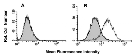
Fig. 1: Binding of A5-PE40 to PSMA expressing cells. Flow cytometric analyses with (A) PSMA negative DU145 cells and (B) PSMA positive C4-2 cells.
